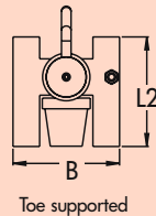
Toe supported
