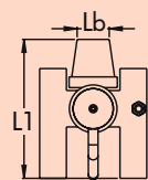
Toe freestanding
